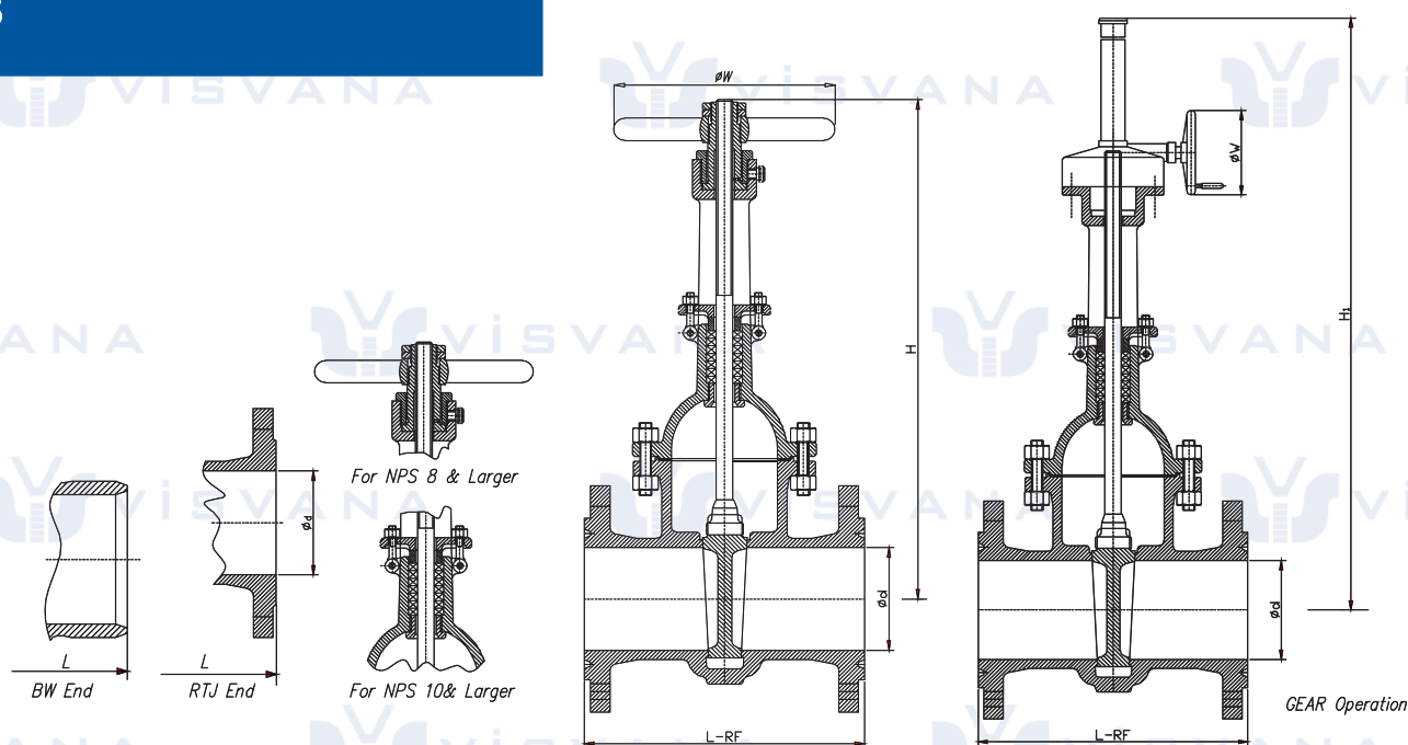
Class 300 & JIS 20K Gate Valve
